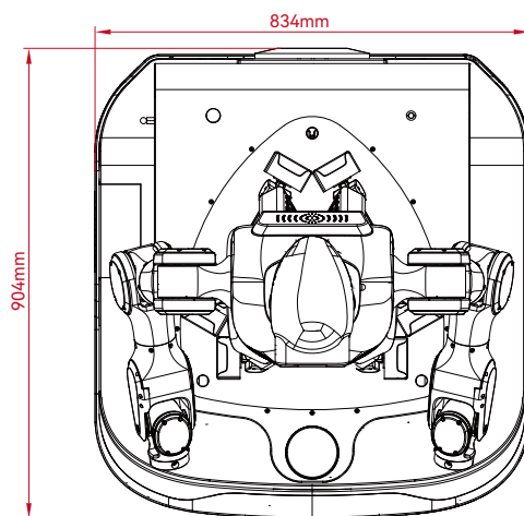
占地面积
